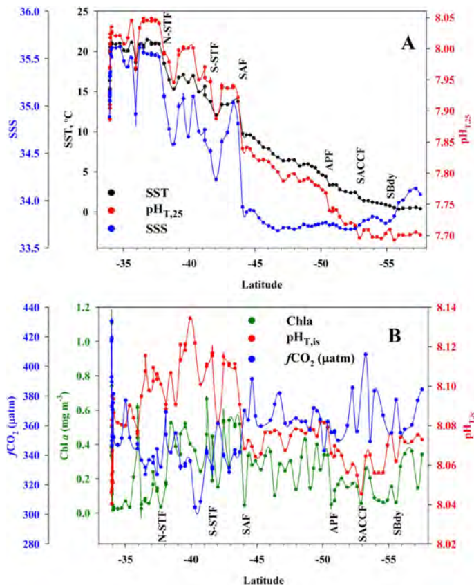
Fig. 2. (A) Sea surface temperature (SST), salinity (SSS) and pH in total scale at 25 °C, pH T,25 , along the cruise track for samples analyzed in the upper 10 m. The figure shows the position of the major frontal zones during the BONUS GoodHope cruise. (B) Surface ocean Chlorophyll-a, partial pressure of CO 2 in seawater expressed as fugacity, fCO 2,sw (μatm) and pH in total scale at in situ conditions, pH T,IS .
