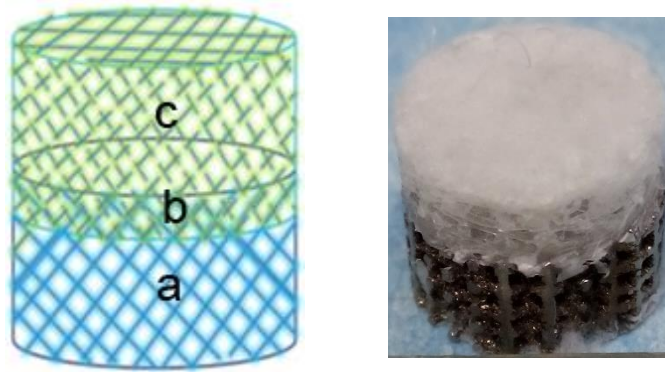
Figure 3. Gradient structure. a: Titanium matrix b: PLA junction c: PLGA infiltrated collagen layer. Courtesy University College London.
