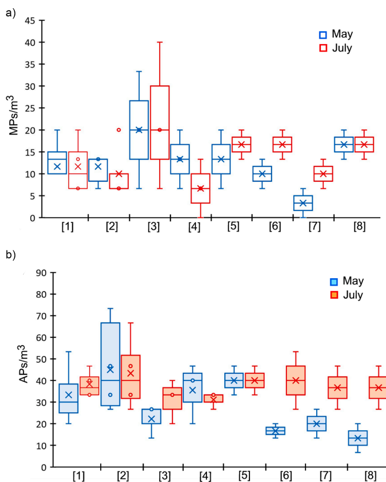
Fig. 2. Number concentration of (a) Microplastics (MPs), and (b) Artificial particles (APs) for the different sampling locations. (The variability among samples taken in the same location is given as inclusive quartiles, the bars representing maximum and minimum values; locations as indicated in Fig. 1; note that the scale for APs is double than that of MPs.).
