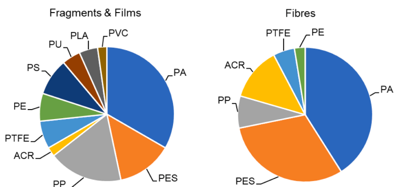
Fig. 3. Chemical composition of fragments/films and fibres for the (84) particles spectroscopically identified as MPs by micro-FTIR. (PA: polyamide; PES: polyester; PP: polypropylene; PE: polyethylene; PTFE: polytetrafluoroethylene; ACR: acrylic polymers; PS: polystyrene; PU: polyurethane; PLA: polylactic acid, PVC: polyvinyl chloride.).
