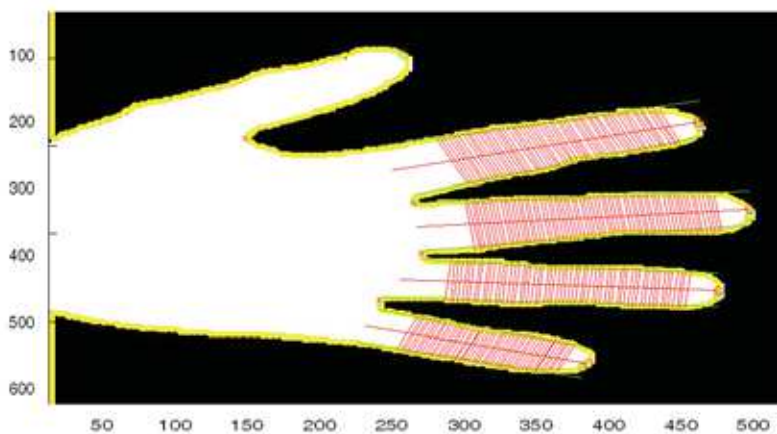
Fig. 4. Feature extraction
