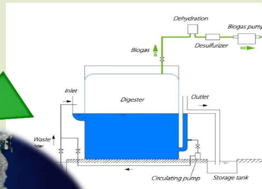
Biodigestor
