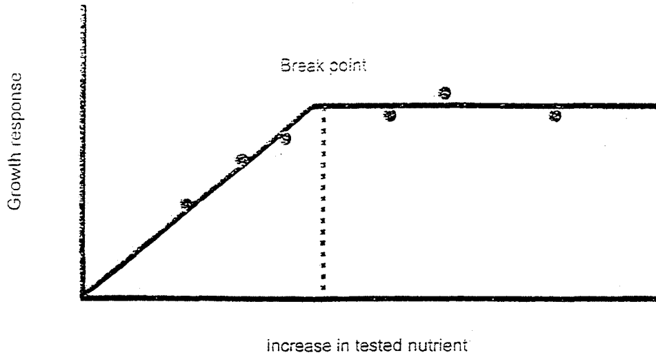
Fig. 1. Broken line model after Robins et al. , 1979.
