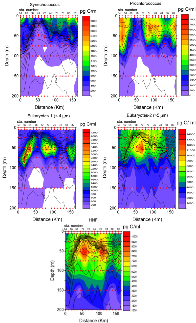
Figure 9: Distribution of the picoplankton and nanoplankton biomasses along the transect, all units are \text{pg C} \cdot \text{ml}^{-1} . (a) Synechococcus, (b) Prochlorococcus, (c) Euk-1, (d) Euk-2 and (e) HNF. See Fig. 3a for the features. Thin black lines are isopycnals, bold black line shows the core of the thermocline; red arrows on the top axis indicate stations position.
