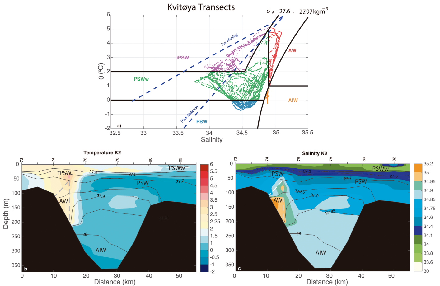
Figure 13. (a) Potential temperature/salinity diagram for of all the transects across the Kvitøya Trough. (b) Vertical section of potential temperature (color, °C) overlain by potential density ( \text{kg m}^{-3} , contours) for section K2 across the Kvitøya Trough (see Figure 2 for the location of the section). The AW is delimited by the dashed line. (c) Same as Figure 13b except for salinity.
