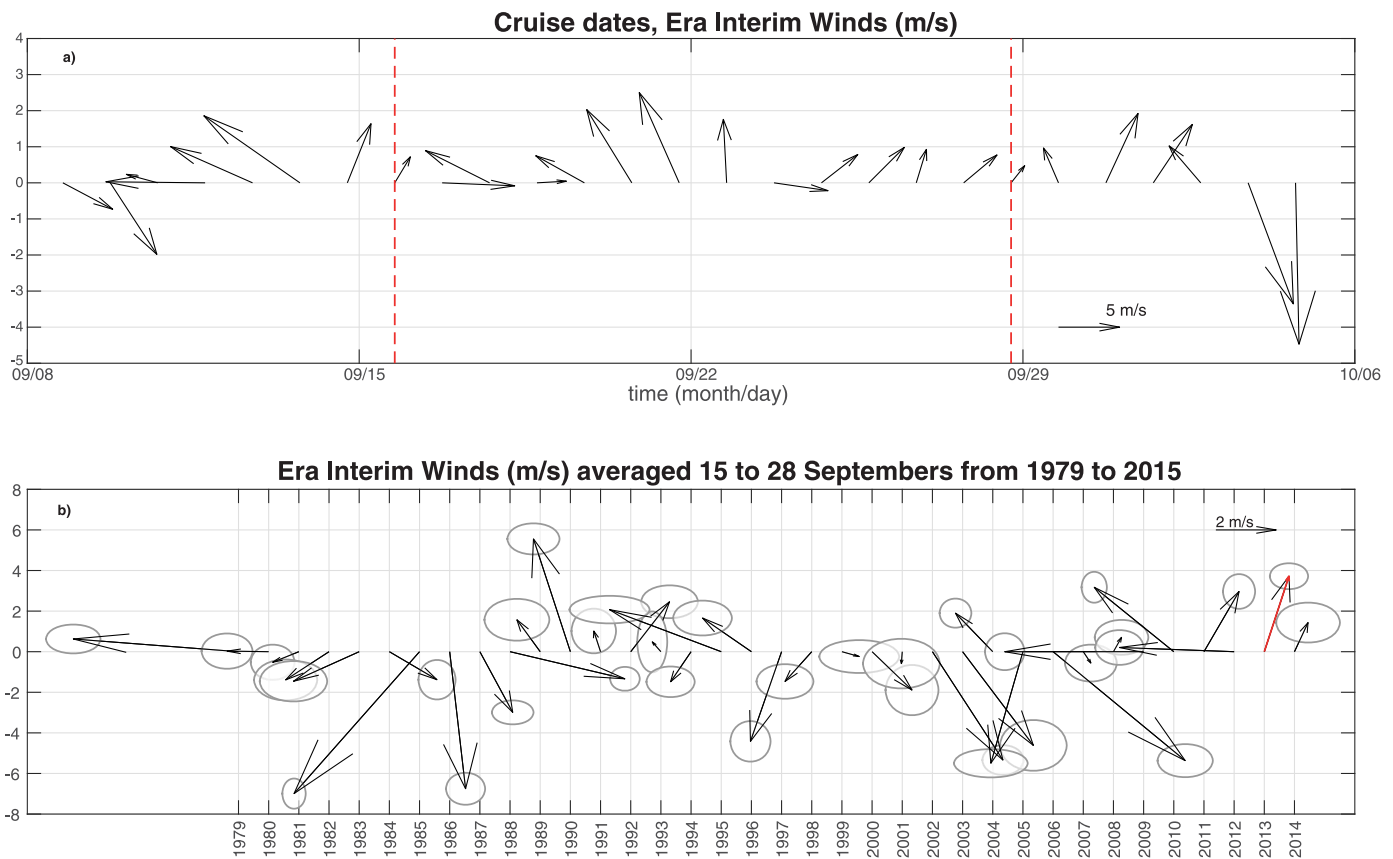
Figure 4. ERA Interim winds at 28.50°N, 81.75°W near the center of our study domain (middle of section B4, see Figure 1). (a) Time series of 10 m winds from 1 week before the cruise to one week after (the period of the cruise is indicated by the red dashed lines). (b) Average 10 m wind vector for 15–28 September (period of the cruise) for each year from 1979 to 2015 together with its standard error ellipse (the cruise year is highlighted as a red arrow).
