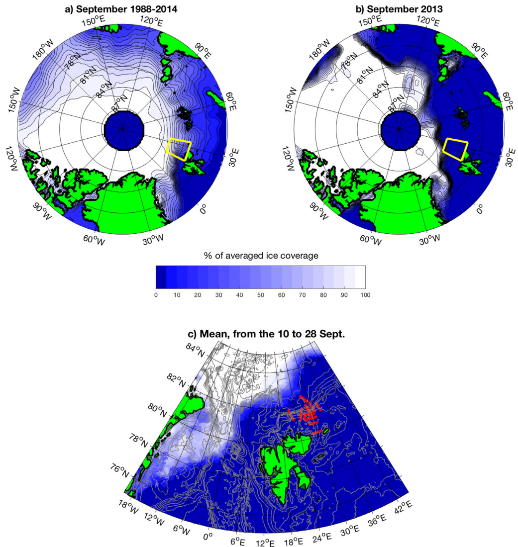
Figure 5. Ice concentration from SMMR, SSMI/I-SSMIS version 1 averaged for (a) September 1988–2014 and (b) September 2013. The yellow box indicates the A-TWAIN study area. (c) Enlarged view of the A-TWAIN study area showing the average ice concentration from MASAM2 during the time of the cruise. Red dots indicate the cruise stations and gray contours represent bathymetry.
