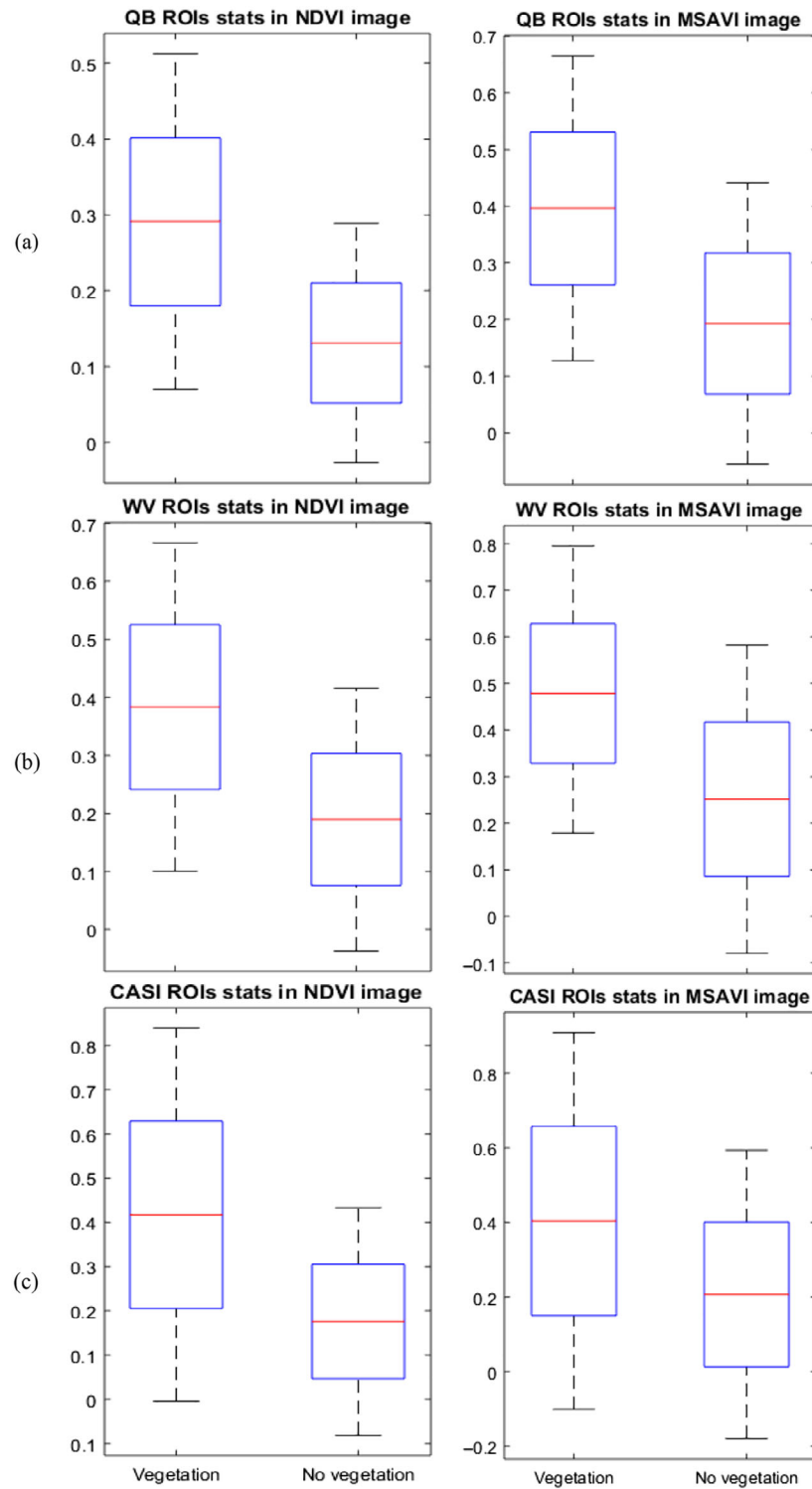
Fig. 8. Normalized difference vegetation index (NDVI) and modified soil-adjusted vegetation index (MSAVI2) boxplot diagrams for: (a) QuickBird (QB), (b) WorldView-2 (WV-2), and (c) compact airborne spectrographic imager (CASI).
