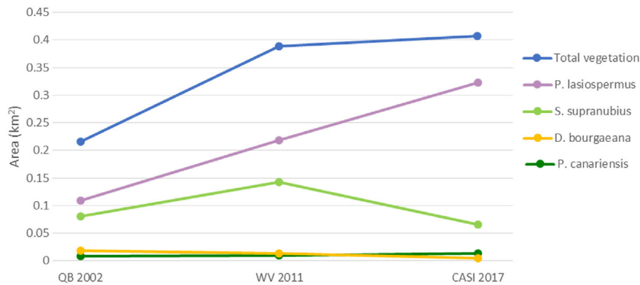
Fig. 10. Vegetated area and plant species coverage in 2002, 2011, and 2017 in the different scenes.
