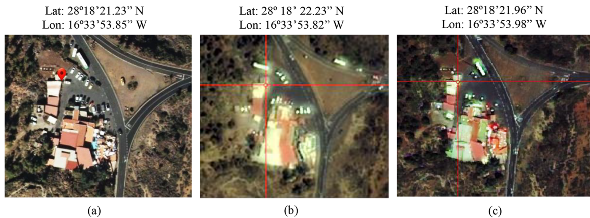
Fig. 6. (a) Orthophotograph of GRAFCAN and images after orthorectification: (b) QuickBird image and (c) WorldView-2 image.
