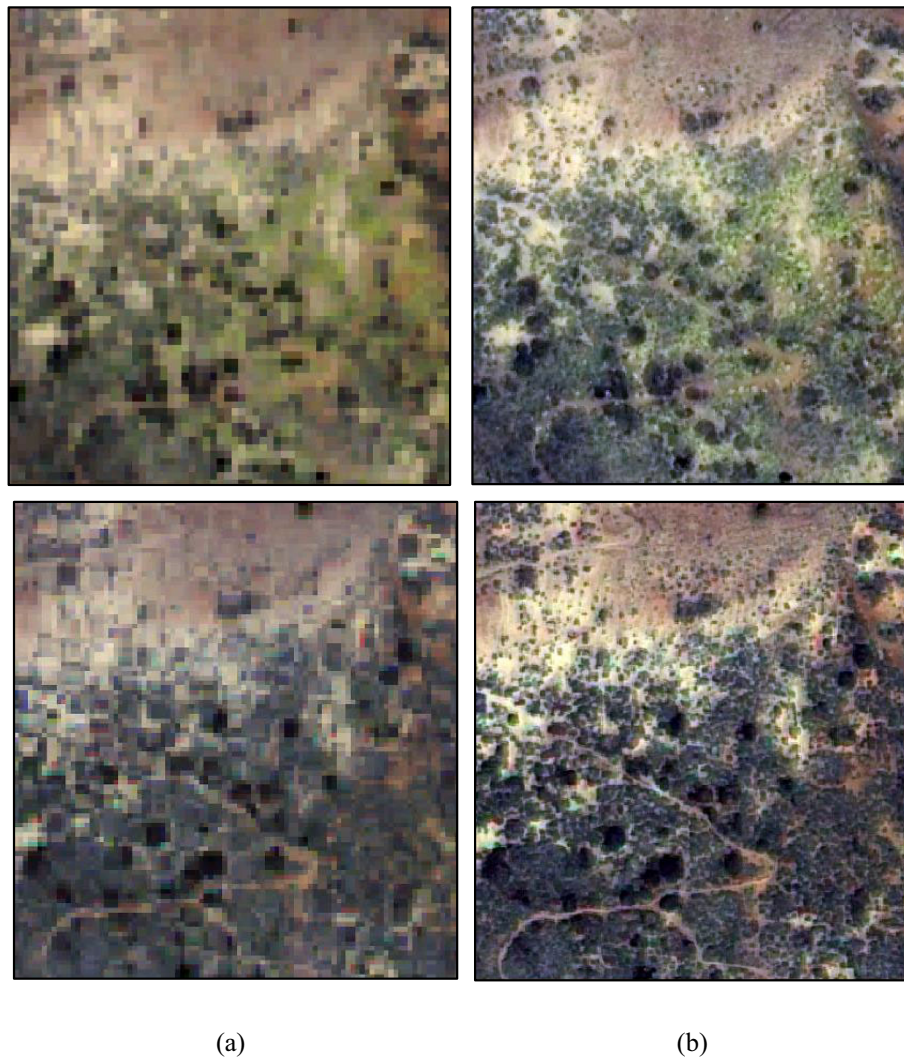
Fig. 5. (a) Original multispectral image and (b) fused image. Top row: QuickBird images. Bottom row: WorldView-2 images.
