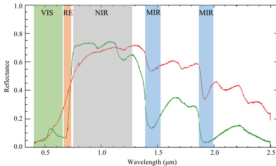
Fig. 4. Vegetation spectral signature. Green signature: healthy vegetation; red signature: dry vegetation. Shaded areas: VIS, visible wavelength corresponding to the chlorophyll peak; RE, red edge; NIR, near-infrared wavelength corresponding with cell structure; MIR, middle infrared corresponding to the water absorption wavelengths.
