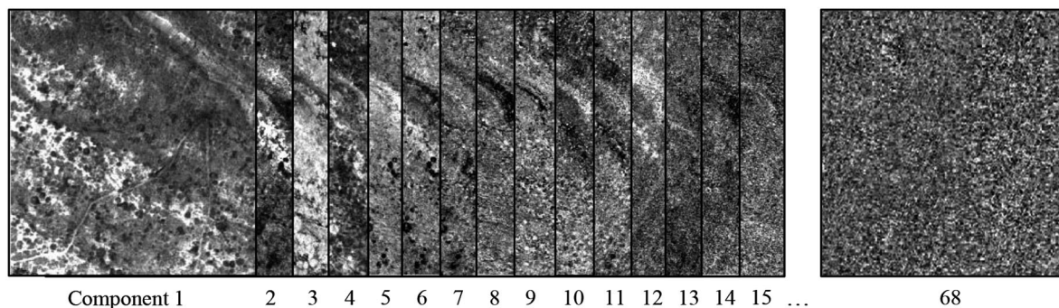
Fig. 7. Minimum noise fraction (MNF) components of the compact airborne spectrographic imager (CASI) image.
