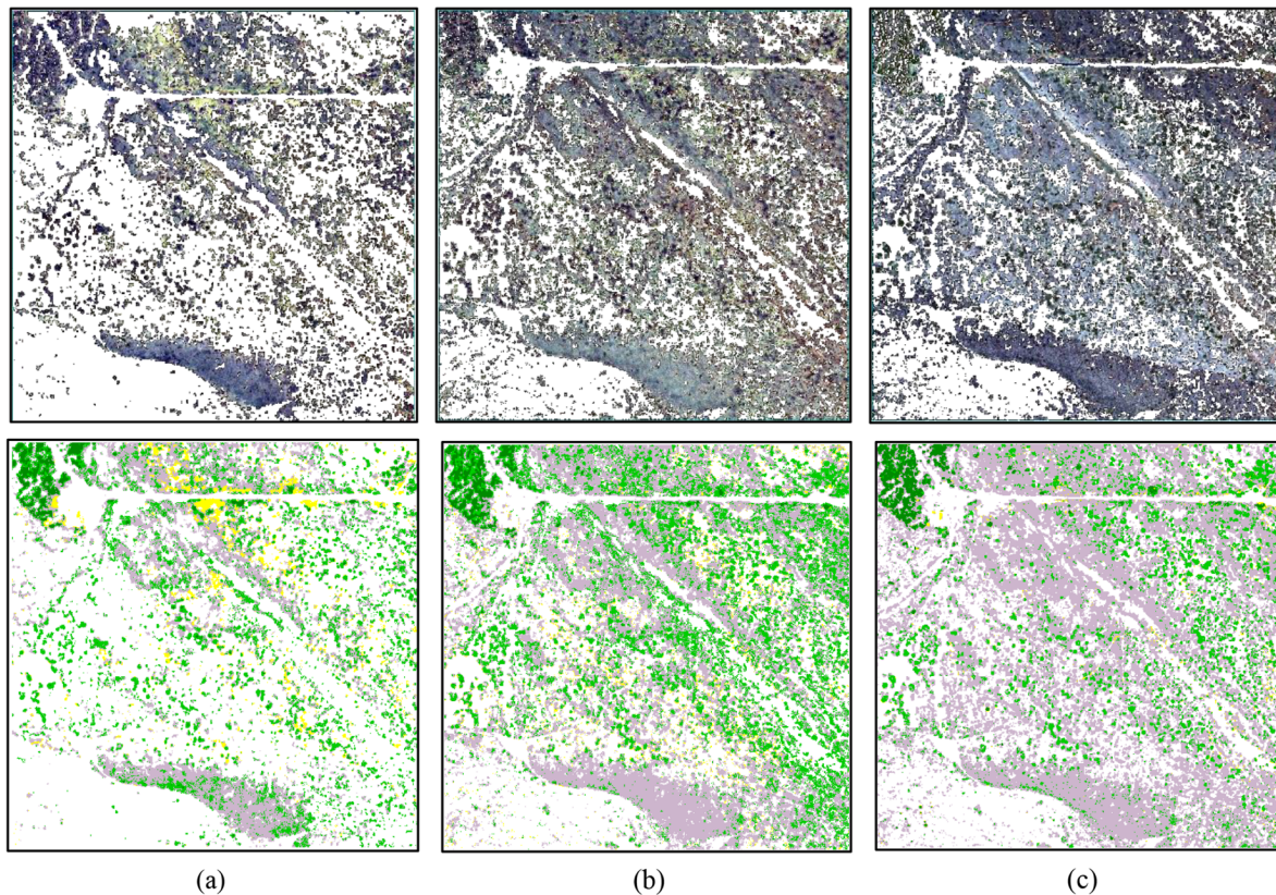
Fig. 9. Top row: Masked and pre-processed images: (a) QuickBird (QB), (b) WorldView-2 (WV-2), and (c) compact airborne spectrographic imager (CASI). Bottom row: Classification maps: (a) QuickBird, (b) WorldView-2, and (c) compact airborne spectrographic imager (CASI) imagery (light green, Spartocytisus supranubius ; dark green, Pinus canariensis ; violet, Pterocephalus lasiospermus ; yellow, Descurainia bourgaeana ).
