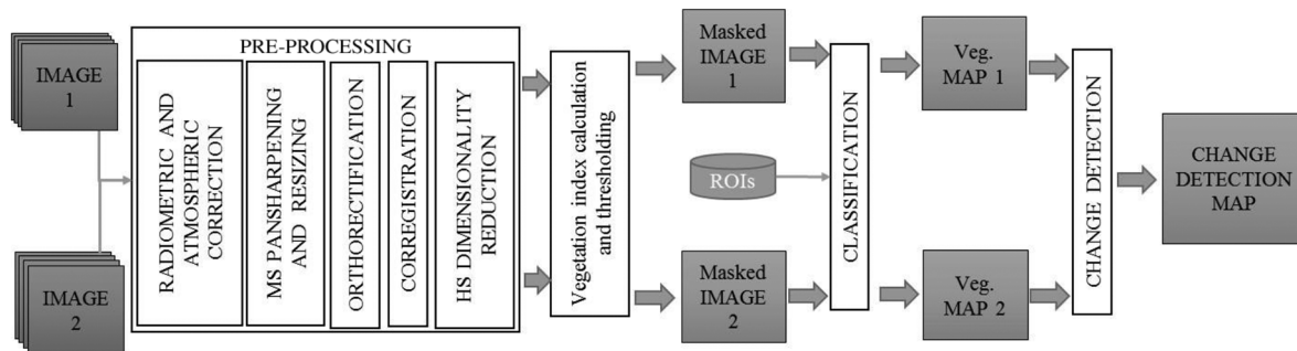
Fig. 3. Diagram followed in the change detection study.
