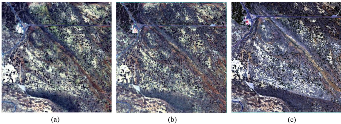
Fig. 2. Remote sensing imagery in RGB color composite: (a) QuickBird of 2002 (R: 3, G: 2, B: 1); (b) WorldView-2 of 2011 (R:5, G: 3, B: 2); (c) compact airborne spectrographic imager (CASI) of 2017 (R:29, G: 20, B: 12).
