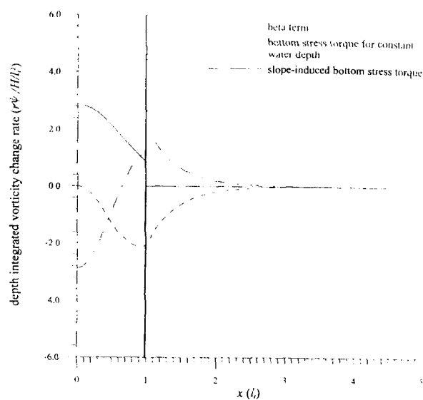
FIG. 6. Depth-integrated vorticity budget for l_s = 2.4l_i as inferred from Eq. (45).
