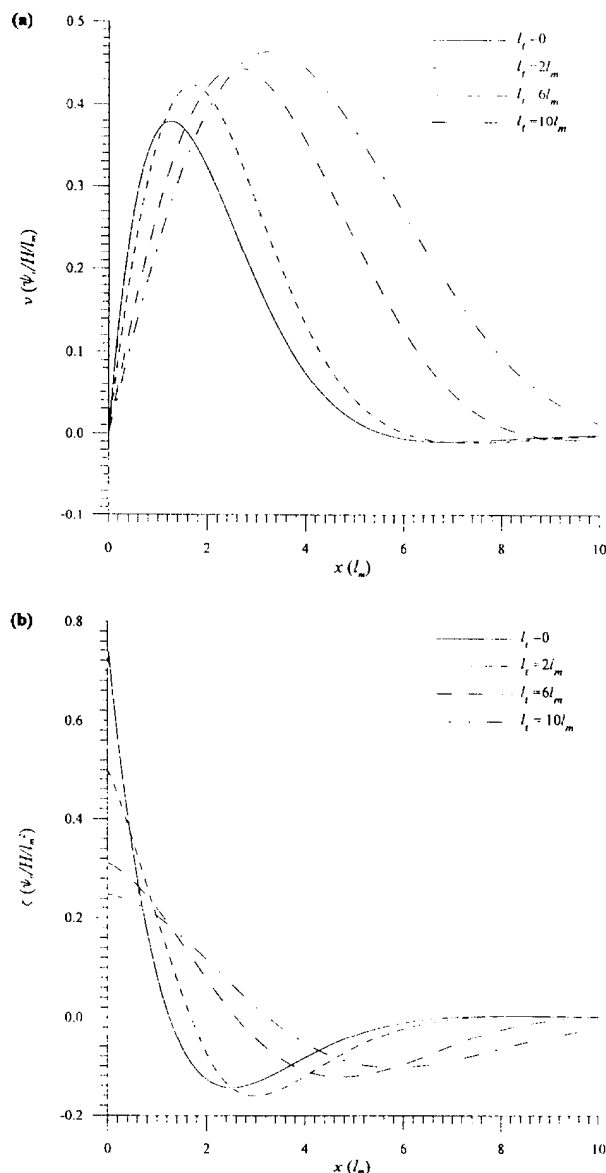
FIG. 3. Zonal structure of (a) velocity and (b) vorticity for l/l_m = 0, 2, 6, 10 , and l_t = l_m as inferred from Eq. (33).
