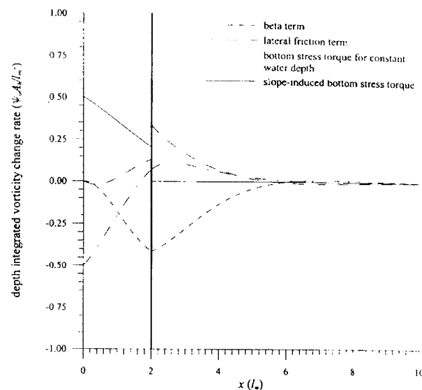
FIG. 4. Depth-integrated vorticity budget for l_t = 2l_m and l_t = l_m as inferred from Eq. (33).
