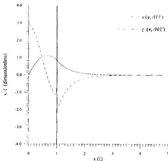
FIG. 5. Zonal structure of velocity and vorticity when l_s = 2.4l_i as inferred from Eq. (45).
