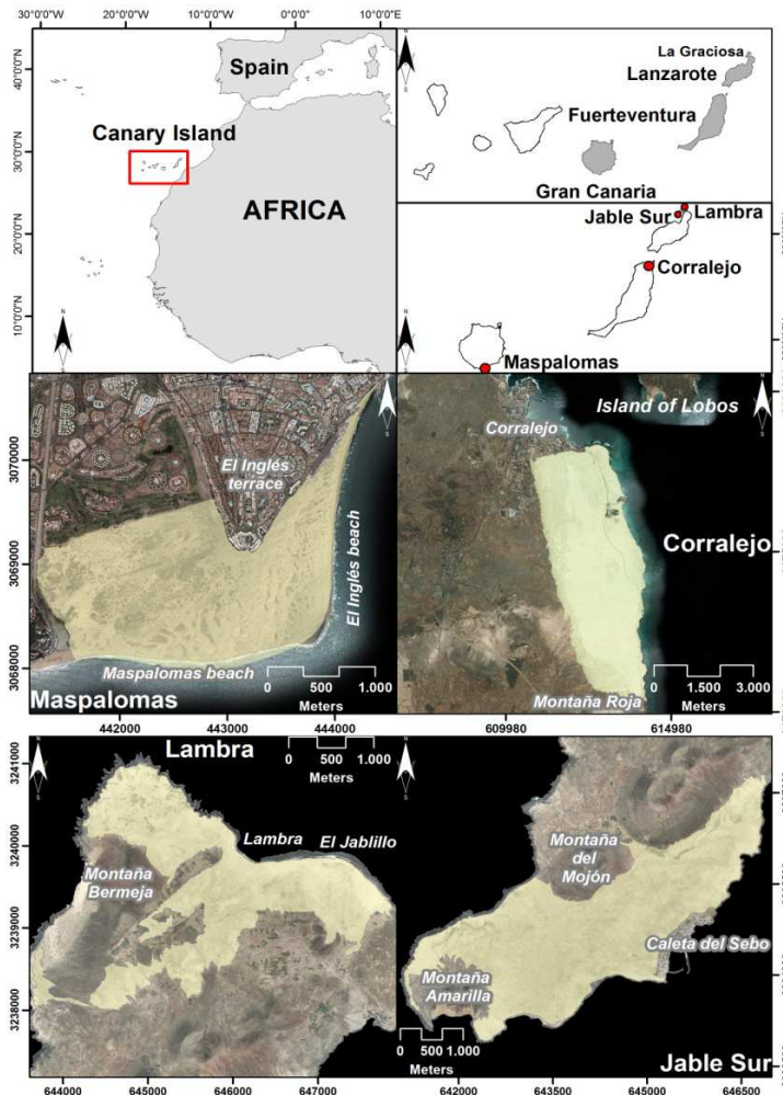
Figure 1: The four arid aeolian sedimentary systems in the Canary Islands.
