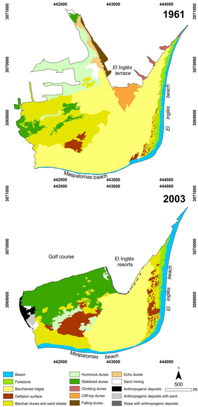
Figure 2: Landform changes in Maspalomas (1961- 2003).
