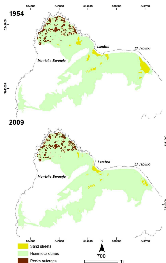
Figure 4: Landform changes in Lambra (1954- 2009)
