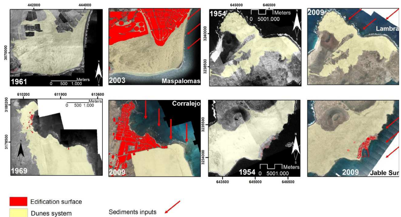
Figure 6: Evolution of the surface area occupied by buildings in aeolian sedimentary systems. Sediment input areas are indicated.
