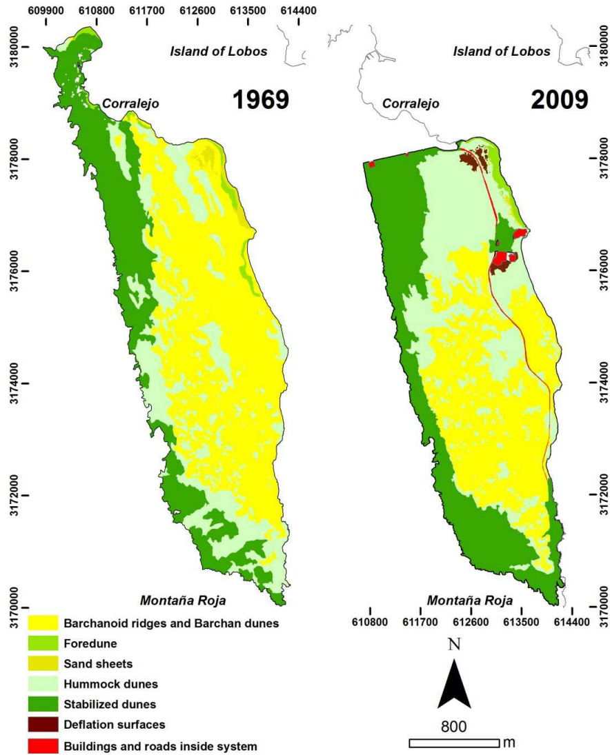
Figure 3: Landform changes in Corralejo (1969-2009).
