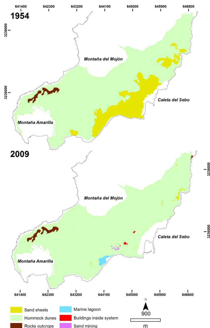
Figure 5: Landform changes in Jable Sur (1954- 2009).
