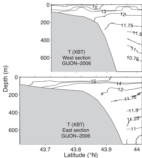
FIG. 9. – Vertical sections of temperature ( ^{\circ}\text{C} ) measured by XBTs during the GIJON-2006 field exercise in the western and eastern sections.
