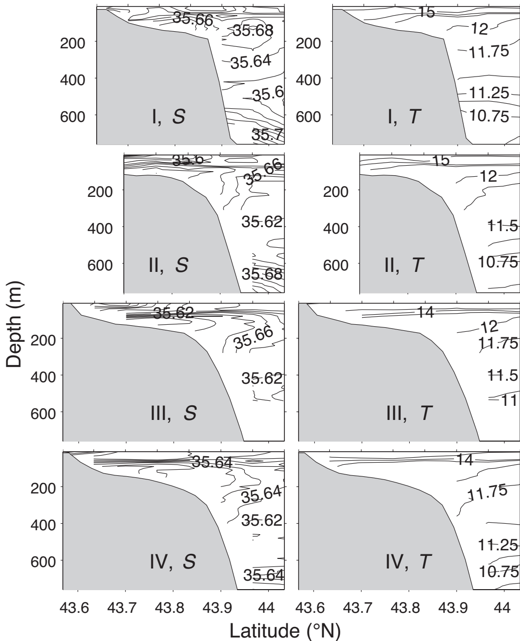
FIG. 10. – Salinity ( S , left) and temperature ( T , right) vertical sections during the ESEOO506-I cruise as a function of latitude. Sections are numbered from west (upper row) to east (lower row) as shown in Figure 2A.
