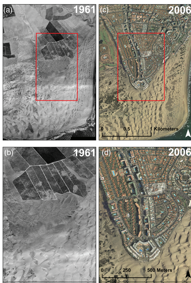
Figure 2. Maspalomas has experienced widespread urbanization between 1961 (a) and 2006 (c). In 1961 (b), climbing dunes were able to bypass the elevated terrace surface, feeding downwind areas with sediment. Following urbanization of the terrace surface (d), this sediment corridor has been disrupted and continual urbanization has further modified the regional airflow dynamics at the Maspalomas dunefield.
