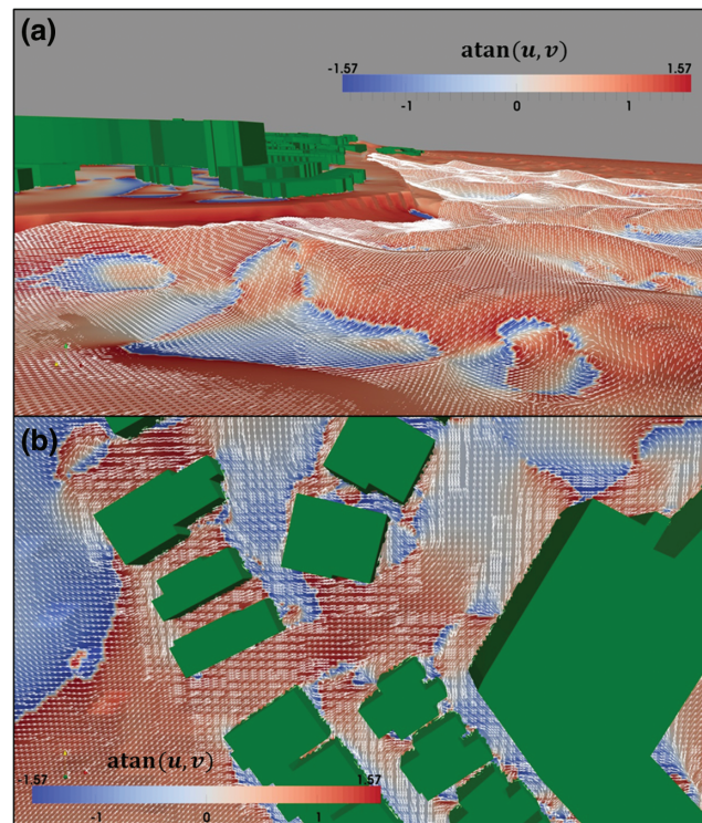
Figure 10. Turbulent flow conditions including counter-rotating vortices represented by surface vectors showing the angle of flow between the streamwise ( u ) and spanwise ( v ) flow components (a, b).
