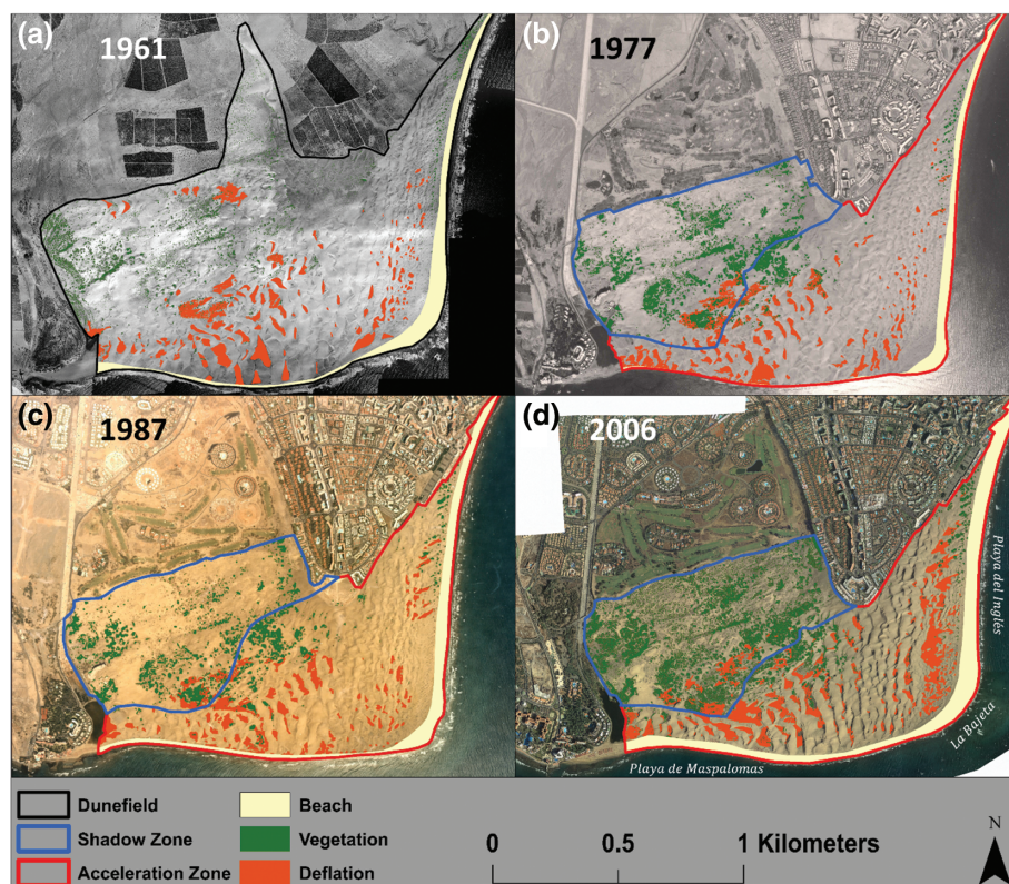
Figure 4. Land cover change occurring at Maspalomas for the years 1961 (a), 1977 (b), 1987 (c), and 2006 (d). Changes in the areal extent of the dunefield, urban shadow zone (i.e., <\delta q' ), acceleration zone (i.e., >\delta q' ), beach, vegetation, and deflation surfaces have changed through time.
