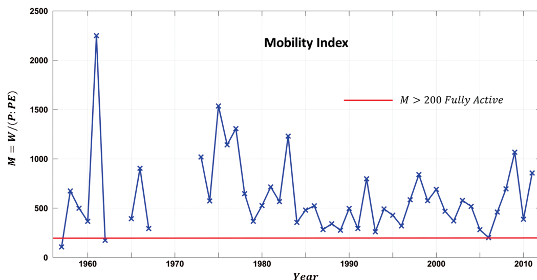
Figure 6. The dune mobility index ( M ) for the Maspalomas dunefield between the years 1957 and 2011. M values largely remain >200 , which are classified as fully active dunes with limited stabilization due to vegetation.
