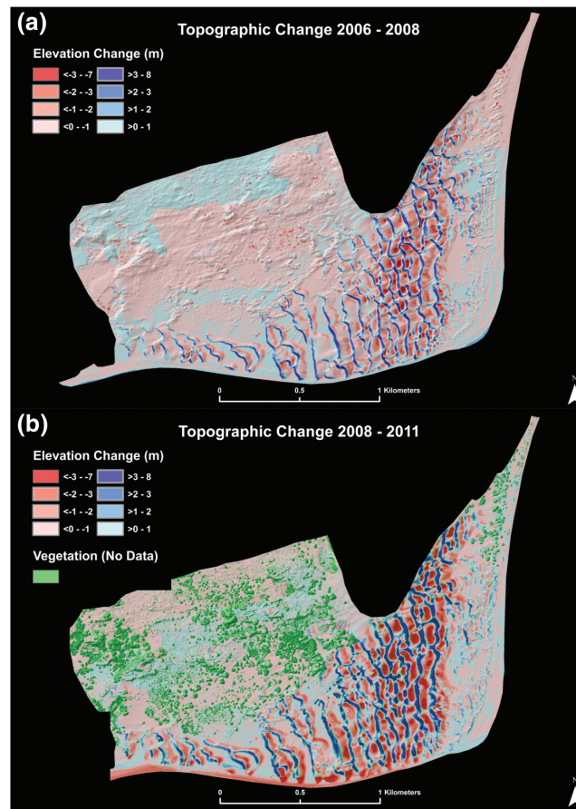
Figure 5. Topographic changes, identified from aerial LiDAR surveys, between the years 2006–2008 (a) and 2008–2011 (b). The 2011 Light Detection and Ranging dataset was unfiltered and vegetation was considered null due to overestimation of the “bare-earth” surface.
