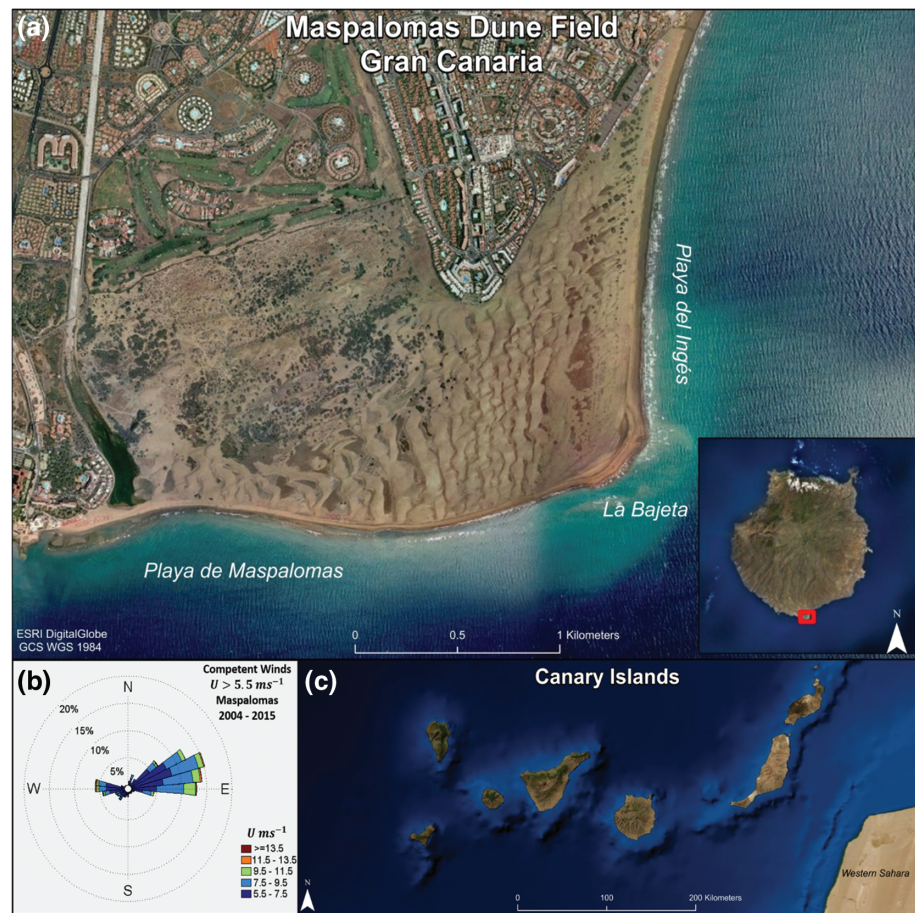
Figure 1. Maspalomas dunefield is located on the southern coast of Gran Canaria, Canary Islands, Spain (a, c). The competent wind regime (i.e., >5.5 \text{ m s}^{-1} ) was recorded at an Agencia Estatal de Meteorología meteorological weather station located 0.6 km to the west of Playa de Maspalomas. The wind regime, between 2004 and 2015, was bi-modal with westerly and easterly wind exceeding threshold values (b).
