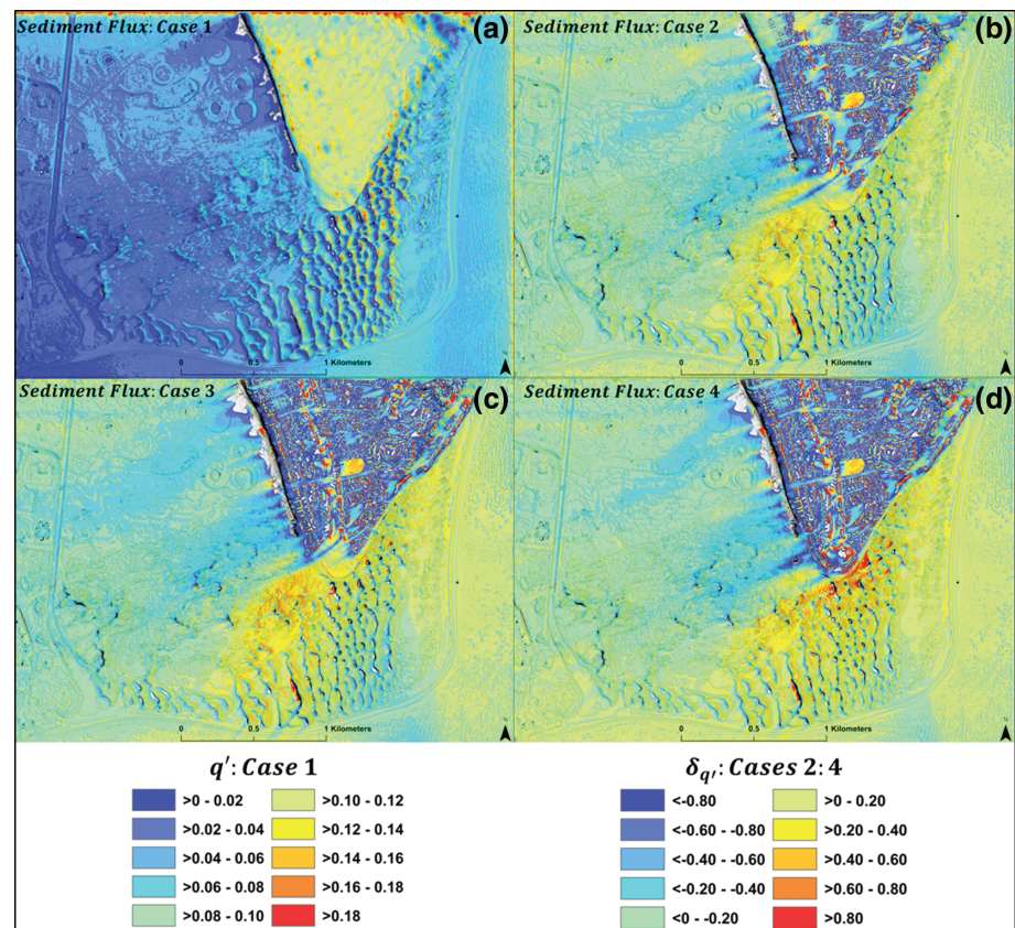
Figure 7. Sediment flux potential ( q' ) during Case 1 and sediment flux perturbation ( \delta q' ) following multiple phases of urbanization for Cases 2–4 (b–d).
