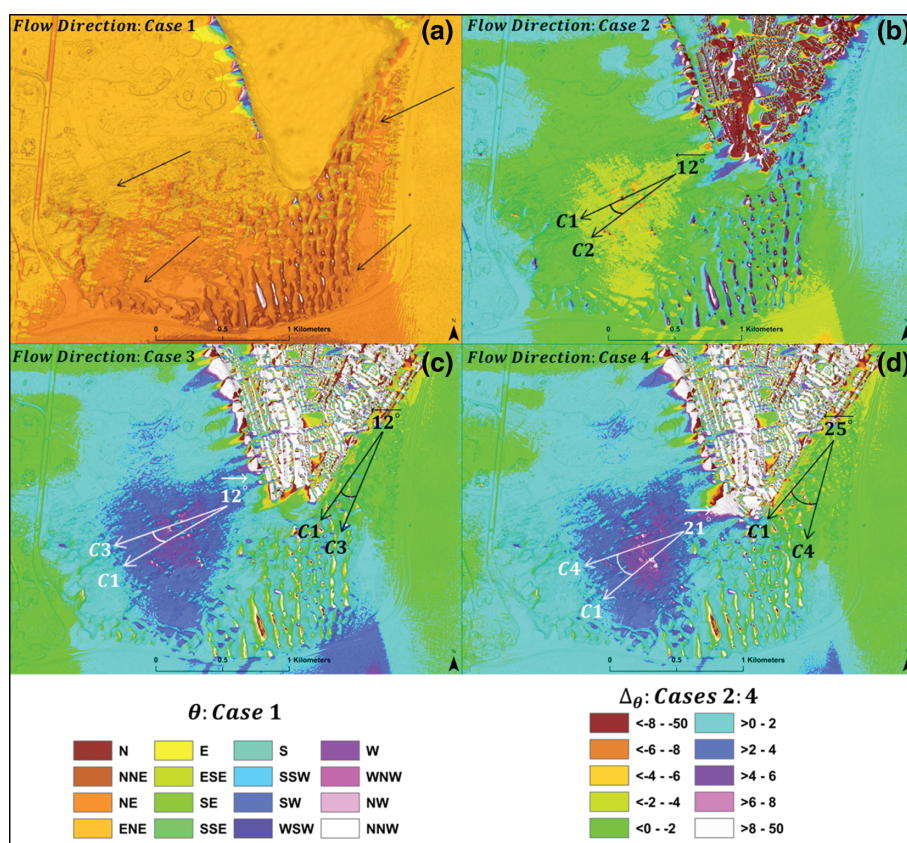
Figure 8. Surface airflow direction ( \theta ) during Case 1 (A) and airflow direction perturbations ( \Delta\theta ) following multiple phases of urbanization for Cases 2–4 (b–d). Arrows indicate the deflection in degrees between the pre-urbanization period (C1) and each subsequent urbanization period (C2–C4).
