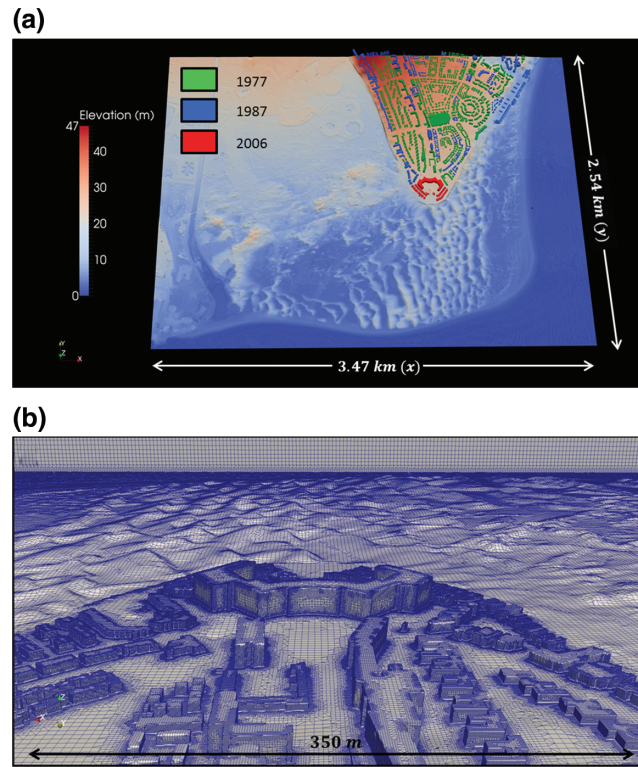
Figure 3. Digital elevation model of the Maspalomas dunefield (2006) with the three major phases of construction across the terrace surface including 1977, 1987, and 2006 (a). A castellated mesh was generated with four levels of progressive cell refinement set toward the coupled model surface, maintaining a representative surface gradient of the complex dune topography and urban geometries (b).
