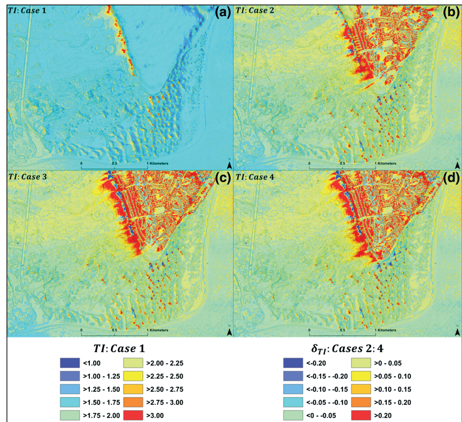
Figure 9. Surface turbulence intensity (TI) during Case 1 (a) and turbulence intensity perturbations ( \delta_{TI} ) following multiple phases of urbanization for Cases 2–4 (b–d).
