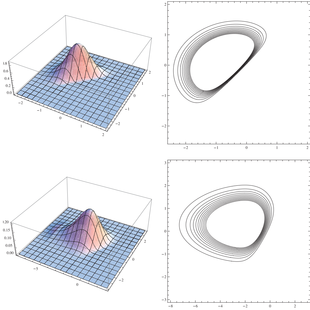
Figure 1: Joint pdf and contour plots of bivariate ordered normal distribution (6) with a_1 = 2 , a_2 = 3 and a_3 = 4 (above) and a_1 = 0.2 , a_2 = 3 and a_3 = 2 (below).
