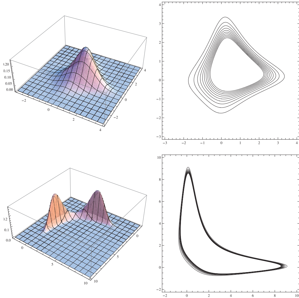
Figure 2: Joint pdf and contour plots of two bivariate distributions with normal conditionals.
