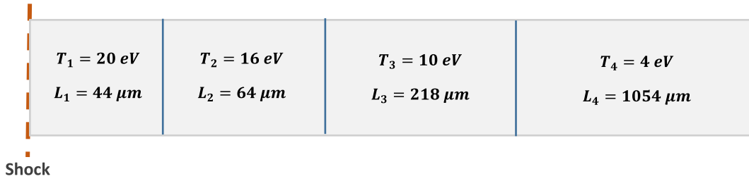
Figure 5. Division of layers of the radiative precursor at t = 8 \text{ ns} . Layer 1 is located closest to shock front, and layer 4 furthest.
