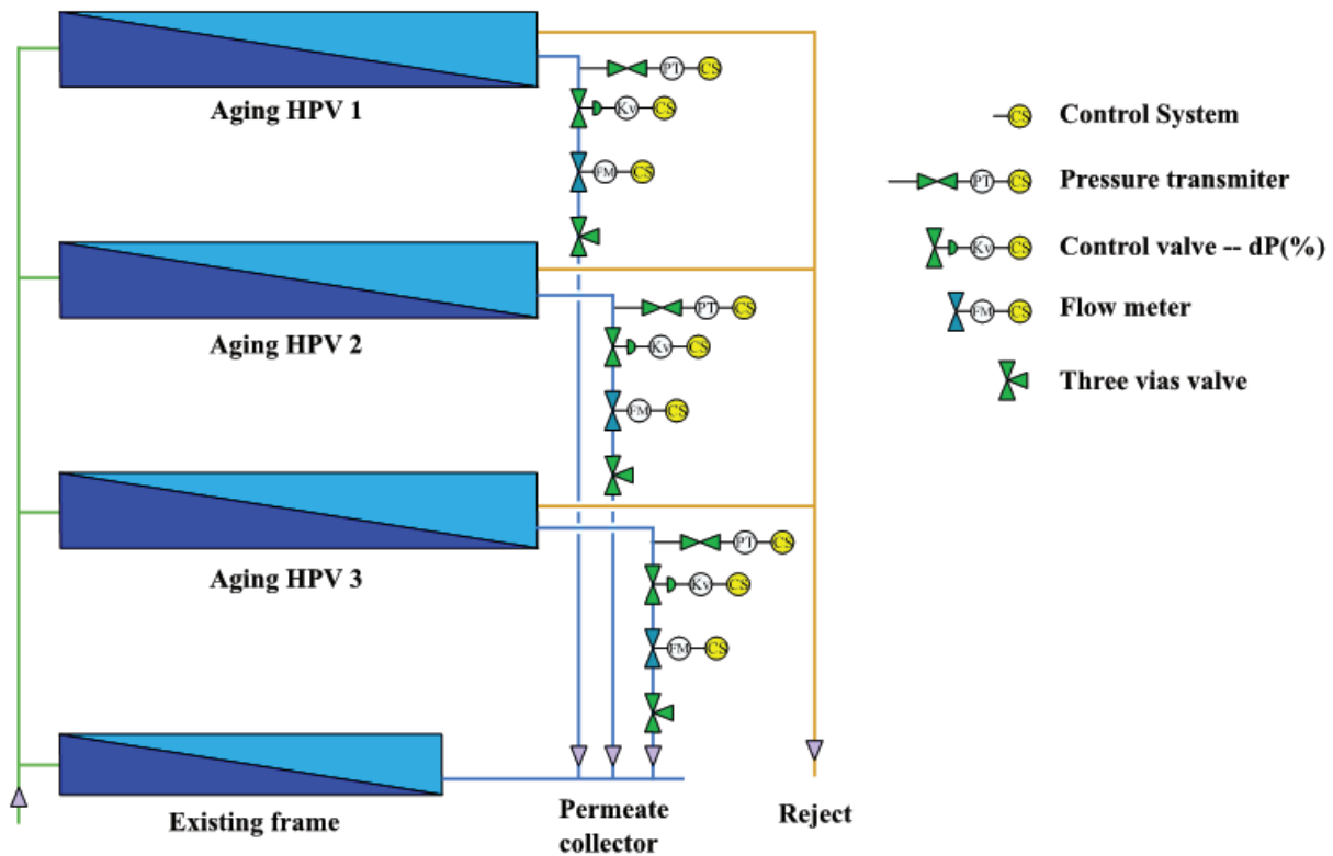
Fig. 2. Aging HPV diagram.
