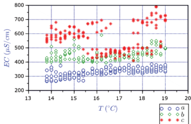
Fig. 4. Permeate conductivity during the aging stage. Comparing permeates conductivity (EC) with TDS [9] we have the following intervals:
