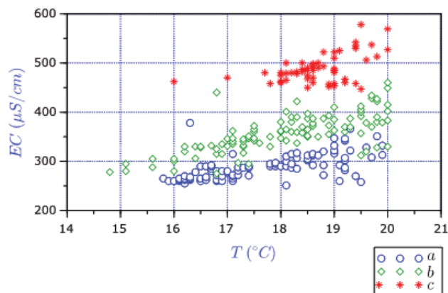
Fig. 6. Permeate conductivity during the Testing stage. Comparing permeates conductivity (EC) with TDS [9] we have the following intervals:
