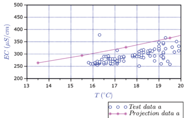
Fig. 7. A-membrane permeate conductivity during the testing stage and projection data.
