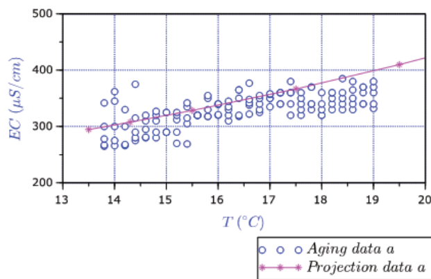
Fig. 5. A-membrane permeate conductivity during the aging stage and projection data.
