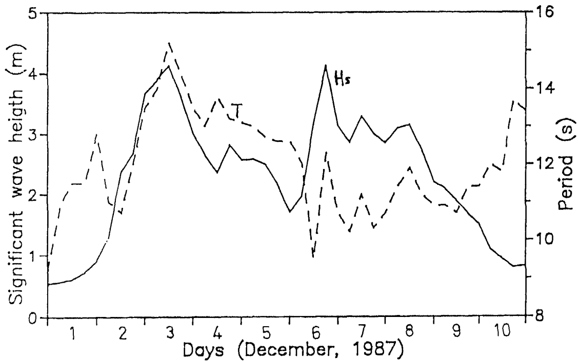
Figure 4. Evolution of significant wave height ( H_s ) and period ( T ) during the first storm.
