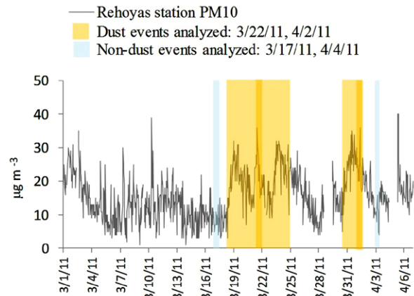
Fig. 2. – Airborne concentration in particles < 10 \mu\text{m} (PM10) measured at Las Rehoayas station, Gran Canaria Island. Selected periods during both dust and non-dust events are highlighted. Las Rehoayas is an urban station placed at 86 m.a.s.l in the northeast of Las Palmas de Gran Canaria (source: Formulario de Datos Históricos de la Red de Control y Vigilancia de la Calidad del Aire, Gobierno de Canarias ; http://www.gobiernodecanarias.org/medioambiente/calidaddelaire/datosHistoricosForm.do ).
