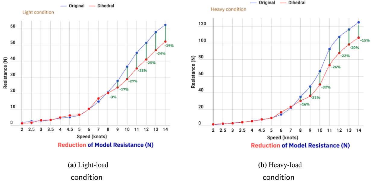
Fig. 8. Total resistance comparison between original and dihedral bulbous bow configurations: (a) Light-load condition; (b) Heavy-load condition.
