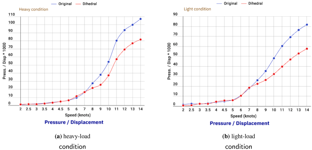
Fig. 9. Pressure resistance comparison for the original and dihedral bulbous bow configurations: (a) Heavy-load condition; (b) Light-load condition.
