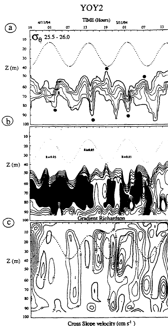
FIG. 3. – Same caption as Figure 2 but for YOY2 time series.
