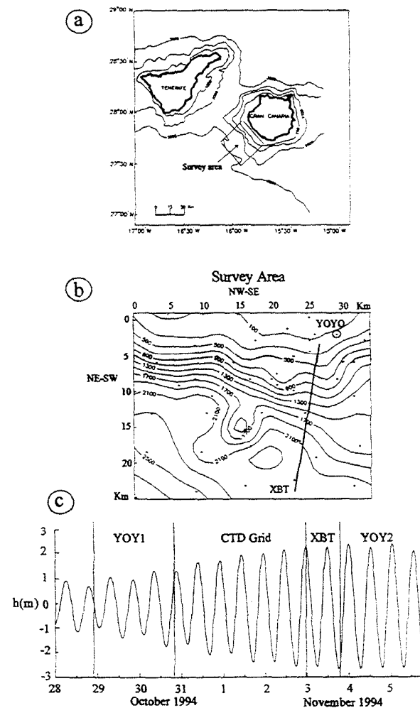
FIG. 1. – (a) Central region of the Canary Archipelago and area of study. (b) Survey area bathymetry, depth contours are marked in meters, the dots indicate CTD stations, the solid line indicates the fast XBT transect, and circle dot shows the position of the fixed sampling location. (c) Survey legs with superimposed barotropic tide amplitude.
