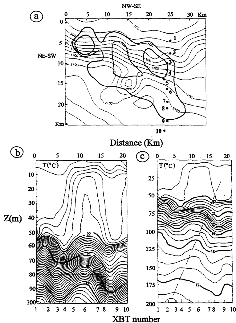
FIG. 6. – (a) Location of the fast XBT section, (b) temperature section down to 100 m, (c) temperature section down to 200 m. In (b) and (c) the bold contours are drawn every 1^{\circ}\text{C} . In (c) the thin broken line joins points of equal phase.
