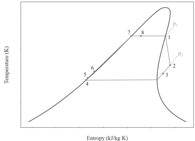
Fig. 2. Temperature-entropy diagram of the subcritical ORC with retrograde fluid.
