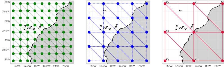
Fig. 3. The mesh nodes are organized into three distinct resolution levels: the finest level on the left ( M^2 , green) consists of 56 nodes, the intermediate level in the middle ( M^1 , blue) includes 16 nodes, and the coarsest level on the right ( M^0 , red) comprises 9 nodes.
