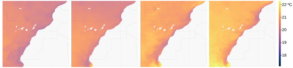
Fig. 2. Several samples of the L4 dataset. These images are examples of the SST on different days of 2020, corresponding to January, April, July, and October, respectively. Colors represent the sea surface temperature in °C, with bright colors representing higher temperatures.
