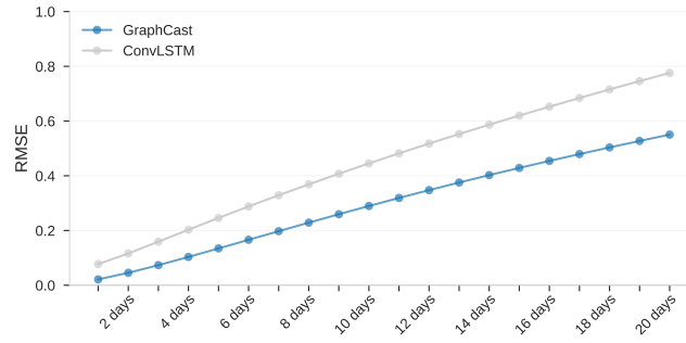
Fig. 5. Comparison of the RMSE values obtained by our model and the ConvLSTM model across a 20-day forecast horizon.
