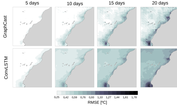
Fig. 6. Spatial distribution of the RMSE for 5-, 10-, 15-, and 20-day lead time forecasts. Results represent daily point-wise averages across the study domain. The graph model yields lower errors in most of the pixels. The highest errors are produced near the coast.
