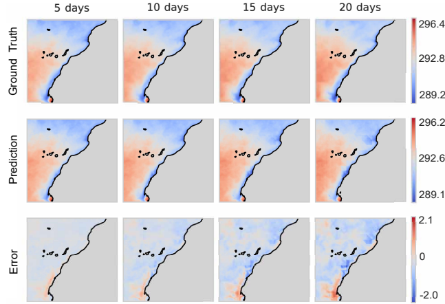
Fig. 4. Forecast comparison for several lead times. The initial date is April 5, 2020, with columns representing forecasts at 5-, 10-, 15-, and 20-day horizons, respectively. The top row shows the ground truth (GT) value for each day, the middle row shows model predictions for the same days, and the bottom row quantifies the error as the difference per pixel between the GT and the prediction.
