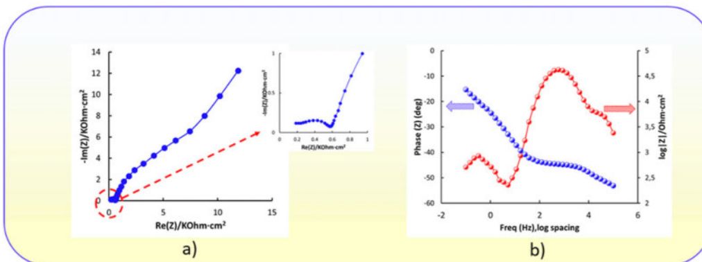
Fig. 4. Impedance diagrams: a) Nyquist; b) Bode-IZI and Bode-phase, for dopped sample in 3.5% NaCl
