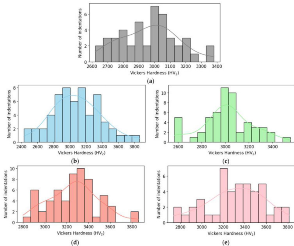
Figure 9. Histogram of Vickers hardness for (a) monolithic B 4 C; (b) B 4 C.05; (c) B 4 C.1; (d) B 4 C.2; and (e) B 4 C.3.
