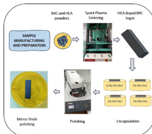
Figure 1. Schematic representation of the material preparation.
