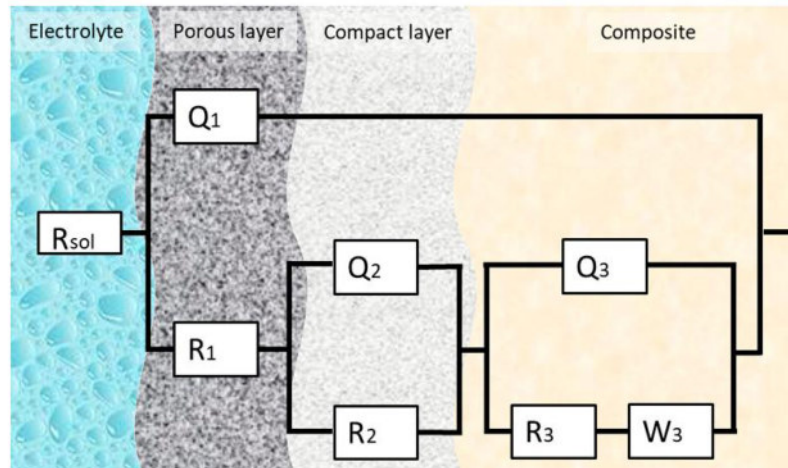
Figure 7. Equivalent circuit R(Q(R(QR)Q(RW))) .
