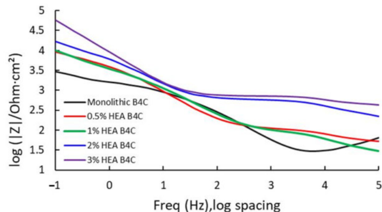
Figure 5. Bode impedance for the studied samples at E_{\text{corr}} after 24 h of immersion in 3.5% NaCl solution.
