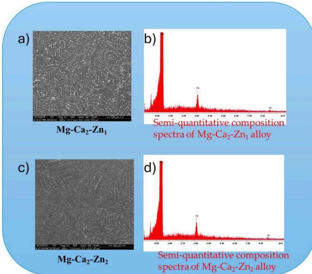
Fig. 2. SEM microstructure of Mg-Ca-Zn alloys.
