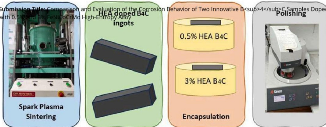
Fig. 1. Fabrication and preparation of the B 4 C samples under study.
