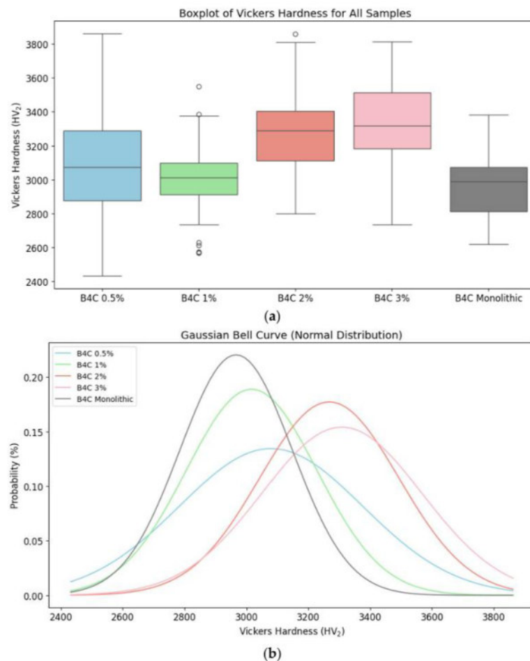
Figure 10. Vickers hardness for B 4 C composites and monolithic sample comparison: (a) distribution of Vickers hardness data through its quartiles; (b) probability distribution of the hardness values.
