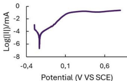
Fig. 1. Linear polarization Rate of doped B 4 C sample.
