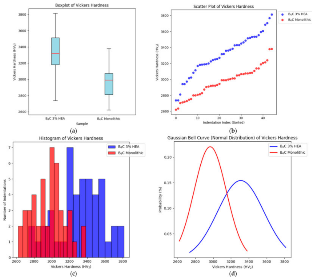
Figure 9. Vickers hardness for both B 4 C monolithic and doped samples comparison: (a) distribution of Vickers hardness data through its quartiles; (b) dispersion of Vickers hardness values; (c) frequency of Vickers hardness values within certain intervals (bins); (d) probability distribution of the hardness values.
