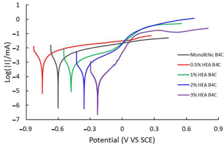
Figure 4. Polarization curve of studied samples in 3.5% NaCl solution.
