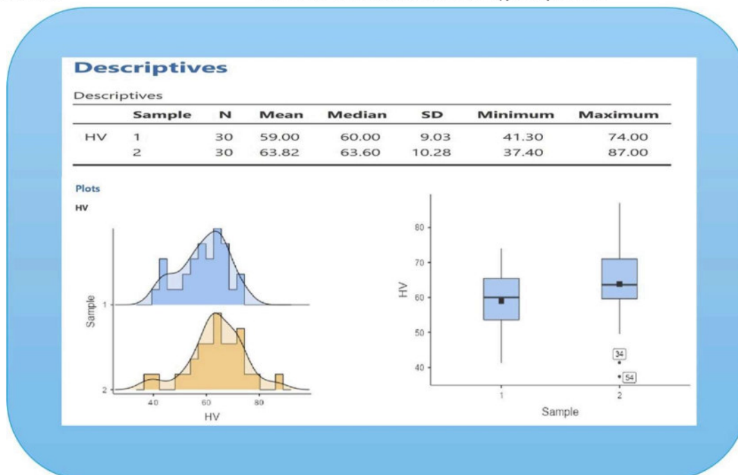
Fig. 3. Microhardness statistics.
