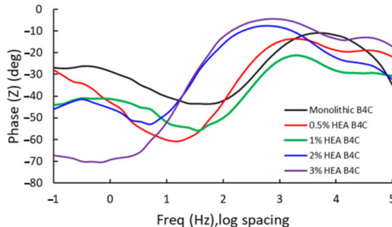
Figure 6. Bode phase for the studied samples at E_{\text{corr}} after 24 h of immersion in 3.5% NaCl solution.
