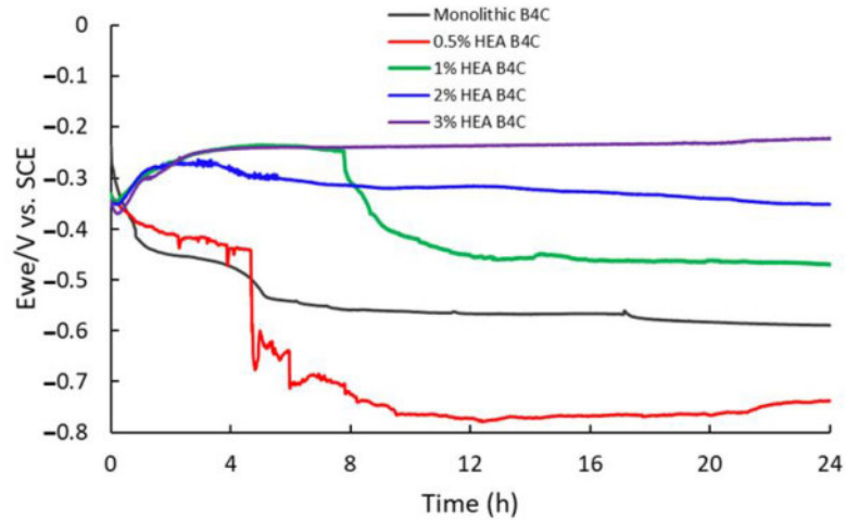
Figure 3. Comparison of corrosion potentials vs. time for 24 h of immersion in 3.5% NaCl solution of studied samples.
