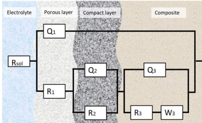
Figure 8. The equivalent circuit for the fitting of the EIS data.
