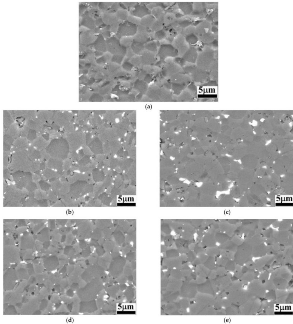
Figure 2. BSE-SEM images of B 4 C and B 4 C-doped composites: (a) monolithic B 4 C; (b) B 4 C.05; (c) B 4 C.1; (d) B 4 C.2; (e) B 4 C.3.
