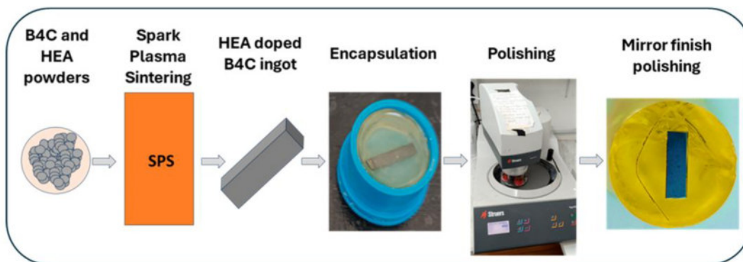
Figure 1. Schematic representation of the material preparation.
