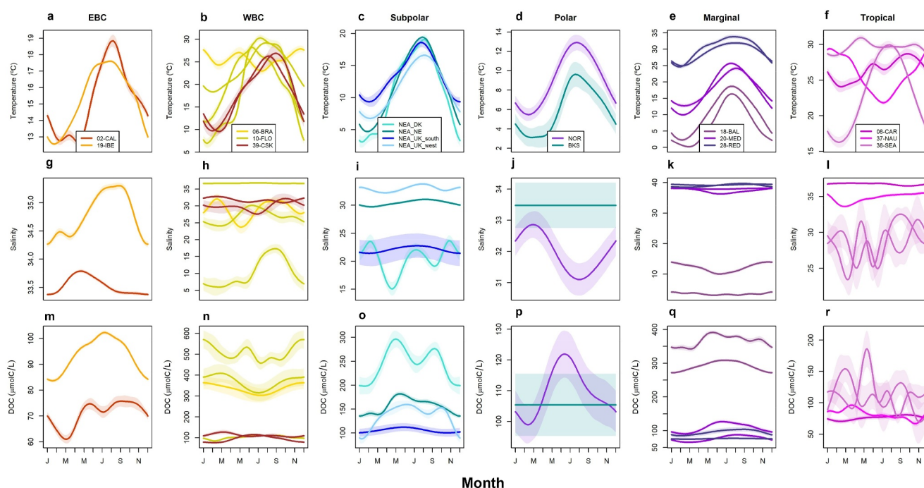
Figure 3. Fitted seasonal trends of temperature (°C) (a–f), salinity (g–l) and dissolved organic carbon (DOC in \mu\text{mol C L}^{-1} ) concentrations (m–r) for regions within the 6 MARCATS segments (EBC, Eastern boundary current margins; WBC, Western boundary current margins; Subpolar margins; Polar margins; Marginal Sea, internal marginal seas; and Tropical margins). Lines in each graph represent the seasonal trend in temperature, salinity and DOC using a generalized additive model (GAM) fit with shaded areas defining 95% confidence intervals of those trends. Please note the difference in scale of the y-axis and that segments were divided into subregions due to differences in the annual trends (i.e., several lines are visible per segment; see text for further details).
