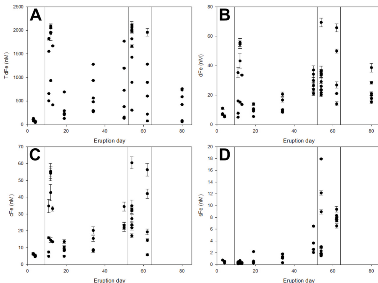
Fig. 2. Temporal evolution of (A) total dissolvable iron (TdFe), (B) dissolved iron (dFe), (C) colloidal iron ( \text{cFe} = \text{dFe} - \text{sFe} ), and (D) soluble iron (sFe) concentrations along the La Palma coast during the Tajogaite eruption. Day 0 corresponds to September 19, 2021. Black vertical lines correspond to the days new deltas started to form (September 28 (day 8), November 10 (day 51), and November 22, 2021 (day 63)).
