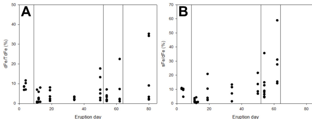
Fig. 5. Temporal evolution of (A) the percentage of dissolved iron content within the readily available iron ( dFe/TdFe ) and (B) the percentage of soluble content within the dissolved phase ( sFe/dFe ). Day 0 corresponds to September 19, 2021.
