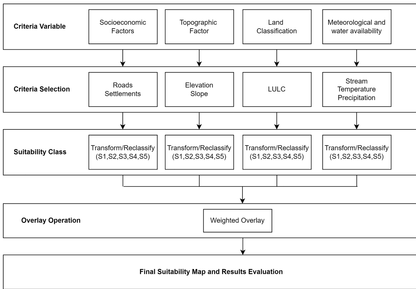
Fig. 5. Methodological flowchart.
