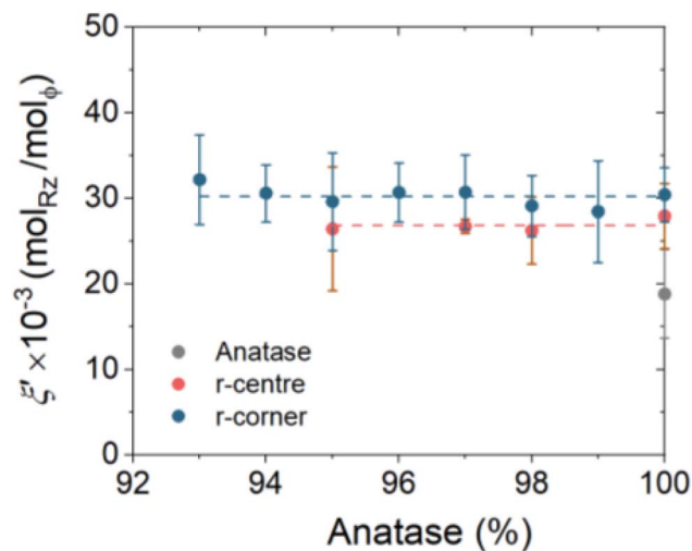
Fig. 8 Apparent photonic efficiencies, \zeta' , given as moles of reduced resazurin per incident photon (units, \text{mol}_{\text{Rz}} \text{mol}_{\phi}^{-1} ) as a function of surface anatase content (>90%, zero-order kinetics) for pure anatase (grey symbols), r-centre (red symbols) and r-corner (blue symbols).
