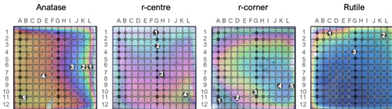
Fig. 1 Photographs of the TiO 2 films, namely pure anatase, r-centre, r-corner and pure rutile, showing enhanced colour fringes, which are related to thickness gradients across the films. Reference 12 × 12-point grids used for XPS analysis are indicated as rows from 1 to 12 and columns from A to L. Selected positions (numbered black circles) indicate analysis points used for further discussion.
