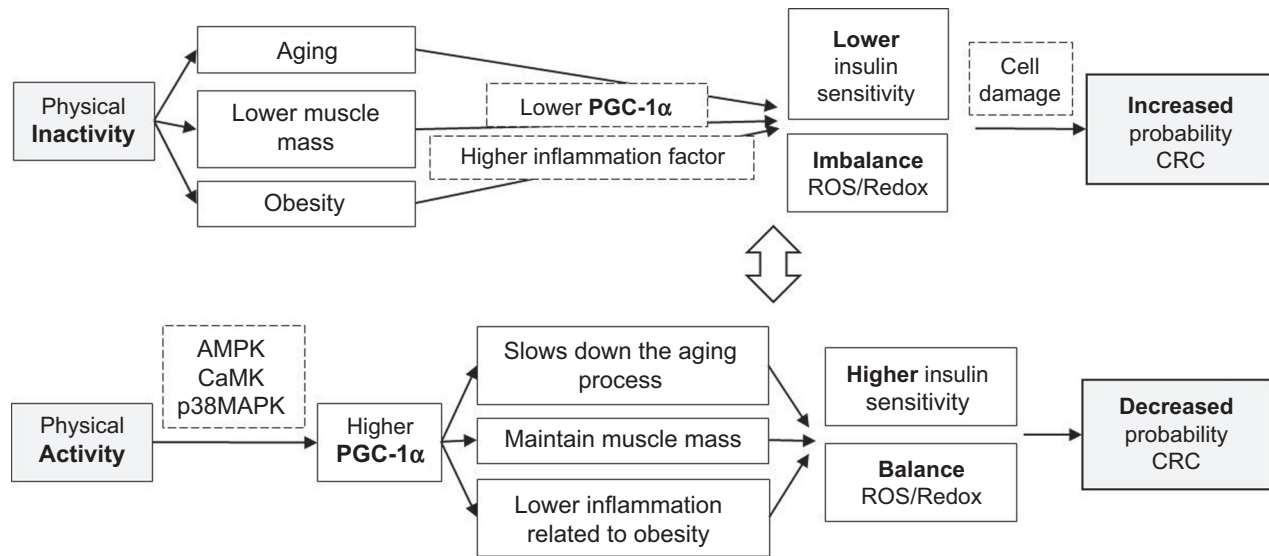
Figure 3. Insulin sensitivity and ROS/Redox balance as a binding factor among physical activity, PGC-1 \alpha , and colorectal cancer. Physical inactivity stimulates the loss of muscle mass, does not contribute to slowing the aging process, and promotes an increase in obesity; it also tends to increase inflammatory factors and tends to be associated with lower levels of PGC-1 \alpha , impacting sensitivity to insulin and ROS/Redox balance. This, in turn, promotes cellular damage and increases the likelihood of colorectal cancer. In the opposite direction, physical activity increases PGC-1 \alpha and interferes with the sensitivity to insulin and balance ROS/Redox positively, thus reducing the likelihood of colorectal cancer.
