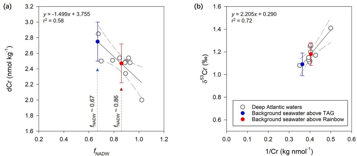
Fig. 3. Relationships (significant at p < 0.05 ; 95 % confidence interval is shown by dashed lines) between (a) dCr and the fraction of NADW ( f_{\text{NADW}} ), and (b) \delta^{53}\text{Cr} and 1/\text{Cr} in deep Atlantic waters (>2000 m, excluding samples collected from within 30 m of the seabed). Open circles represent literature data from Goring-Harford et al. (2018) and Wang et al. (2023). Background seawater Cr concentrations and \delta^{53}\text{Cr} values above the TAG and the Rainbow vent fields are estimated from their known water mass compositions (Table S3). The maximum uncertainties of the background values are \pm 0.25 \text{ nmol kg}^{-1} for dCr and \pm 0.10\% for \delta^{53}\text{Cr} (1.96 times the Root Mean Square Error (RMSE) of the linear correlations).
