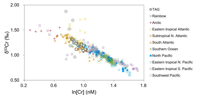
Fig. 6. Cross plot of dissolved δ 53 Cr values versus logarithmic Cr concentration, for new data from this study together with open ocean seawater data from the literature: Scheiderich et al. (2015) (Arctic); Goring-Harford et al. (2018) (eastern tropical Atlantic); Rickli et al. (2019) (Southern Ocean); Moos and Boyle (2019) (North Pacific); Janssen et al. (2020) (North Pacific); Moos et al. (2020) (eastern tropical North Pacific); Huang et al. (2021) (eastern tropical North Pacific); Nasemann et al. (2020) (eastern tropical South Pacific); Janssen et al. (2021) (Southern Ocean, North Pacific, eastern tropical South Pacific, Southwest Pacific, South Atlantic); Janssen et al. (2023) (Southwest Pacific); Wang et al. (2023) (subtropical North Atlantic).
