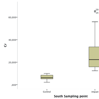
Figure 5.- Mean \pm standard deviation of Cr concentrations at impacted and control sites of SW area.
