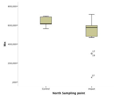
Figure 3.- Mean \pm standard error concentrations of Mn between control and impacted sites at NE area.
