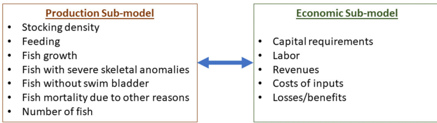
FIGURE 1 Model framework.
