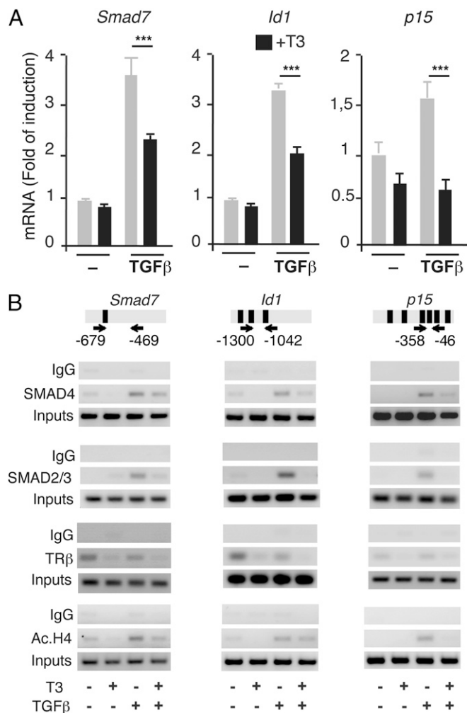
Fig. 6. T3 represses stimulation of endogenous TGF- \beta target genes and inhibits in vivo occupancy of the promoters by SMADs. (A) Level of transcripts for the Smad7 and p15 genes were determined by quantitative PCR in GH4C1 cells treated with T3 for 36 h and TGF- \beta for the last 24 h. The early induction of Id1 mRNA was analyzed after 1 h treatment with TGF- \beta . Data are mean \pm SD. Significance of Bonferroni post hoc test ( n = 3 ) is indicated. (B) ChIP assays were performed with the indicated fragments of the TGF- \beta target promoters that contain SBEs. Location of the primers used is shown with arrows, and the SBEs are depicted as black boxes. Cells were treated for 1 h with T3 and/or TGF- \beta and analyzed by ChIP with nonimmune IgGs, SMAD4, SMAD2/3, SMAD4, TR \beta , and acetylated histone H4 antibodies. One representative experiment of two is shown. The input for each assay is also shown.
