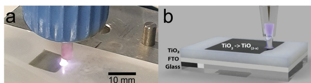
Fig. 1 (a) Photograph of the plasma jet treatment on a titania film showing a sample area of black TiO 2 . (b) Diagrammatic view of the reduction process.
