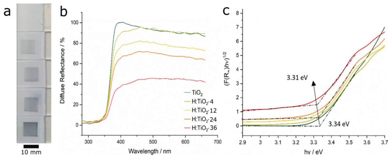
Fig. 2 (a) Photographs of reference sample after consecutive plasma jet passes (from top to bottom, pristine \text{TiO}_2 and \text{H}:\text{TiO}_2\text{-}n with n = 0, 4, 12, 24, 36 s \text{mm}^{-2} ). (b) Diffuse reflectance spectrum of pristine ( \text{TiO}_2 ) and plasma-treated ( \text{H}:\text{TiO}_2\text{-}n ) films upon increasing treatment time with the plasma jet and (c) corresponding Tauc plots of the transformed Kubelka–Munk functions.
