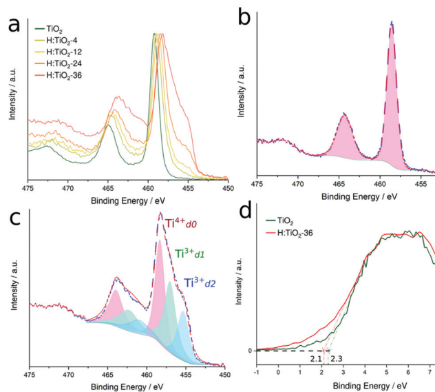
Fig. 3 (a) High resolution Ti 2p XP spectra from pristine and increasingly plasma-treated reduced samples. Peak decomposition analysis of Ti 2p XP spectra is highlighted for pristine (b) and \text{H}:\text{TiO}_2\text{-}36 (c) samples. (d) Corresponding valence bands of pristine and \text{H}:\text{TiO}_2\text{-}36 samples.
