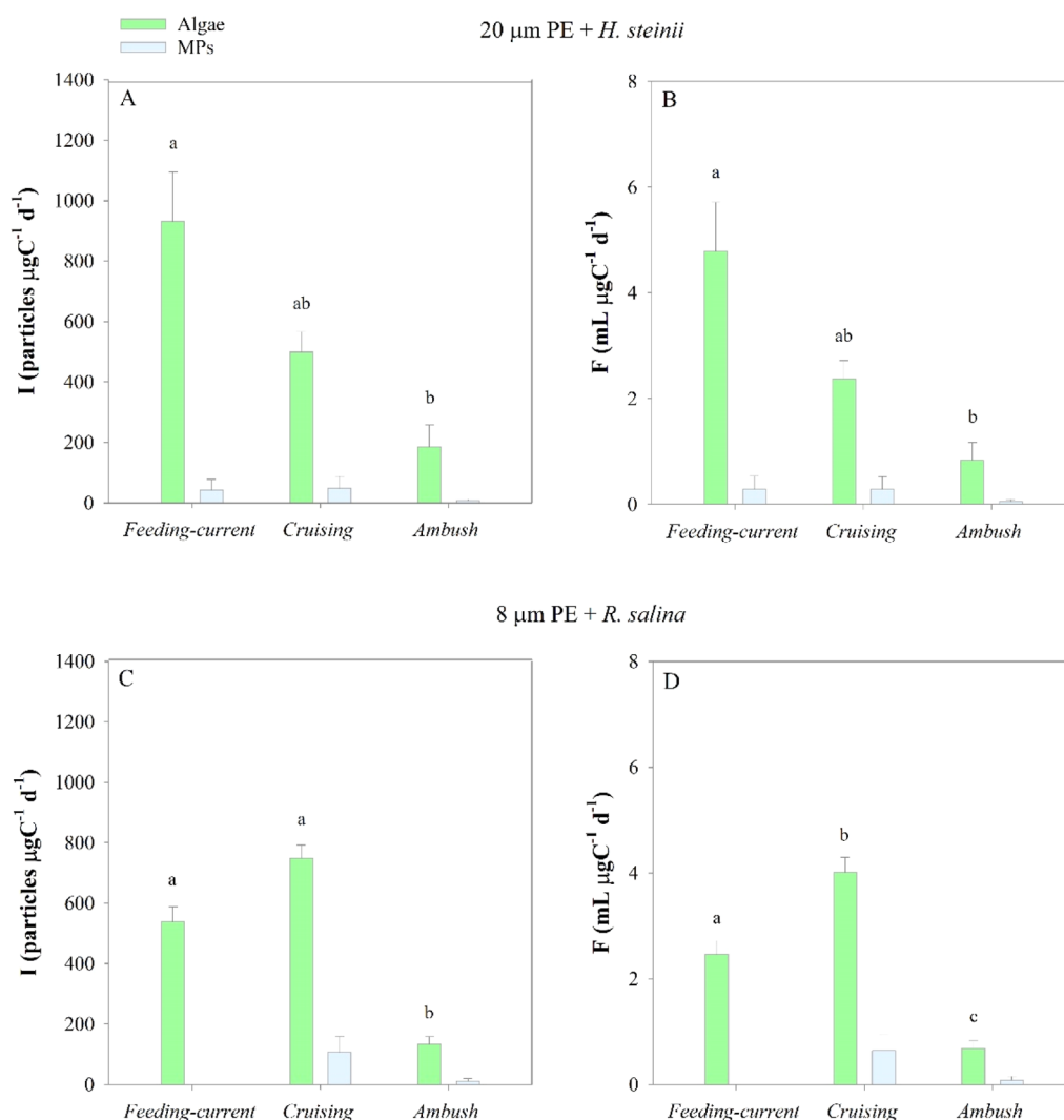
Figure 2. Ingestion (I, particles \mu\text{gC}^{-1} \text{d}^{-1} ) and clearance rates (F, mL \mu\text{gC}^{-1} \text{d}^{-1} ) of algae (green bars) and MPs (blue bars) for the three main feeding behaviors of copepods. Top panels (A,B) show the data for MPs and algae of 20 \mu\text{m} in diameter and the bottom panels (C,D) show the data for 8 \mu\text{m} particles and algae. Data are presented as means of triplicates with the standard error. Asterisks (*) represent a statistically significant difference between algae and MP ingestion or clearance rate within each behavior. Letters indicate significance differences among behaviors.
