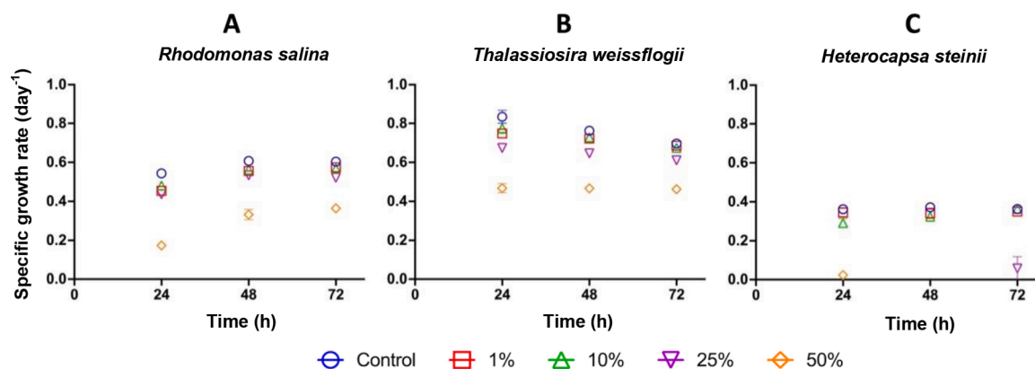
Fig. 2. Specific growth rates ( d^{-1} ) of Rhodomonas salina (A), Thalassiosira weissflogii (B) and Heterocapsa steinii (C) (mean \pm SD) after being exposed to different concentrations of leachates and exposure time. Negative growth rates are not shown.
