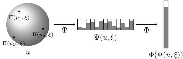
Figure 3. To evaluate the classifier on a test image u , for an hypothetical pose \xi , the algorithm first computes the feature vector \Psi(u, \xi) , and then the response of the predictor \Phi(\Psi(u, \xi)) .
