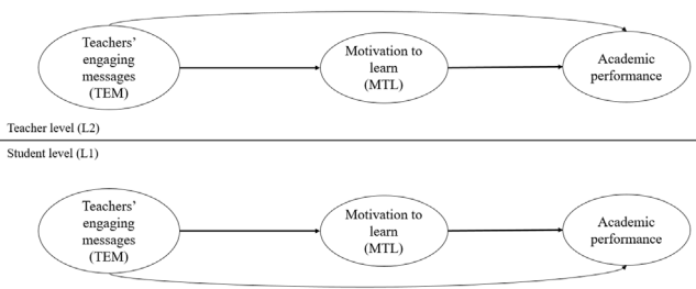
Figure 2. Proposed ML-SEM.
