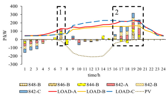
Fig. 7 ESS output profiles
