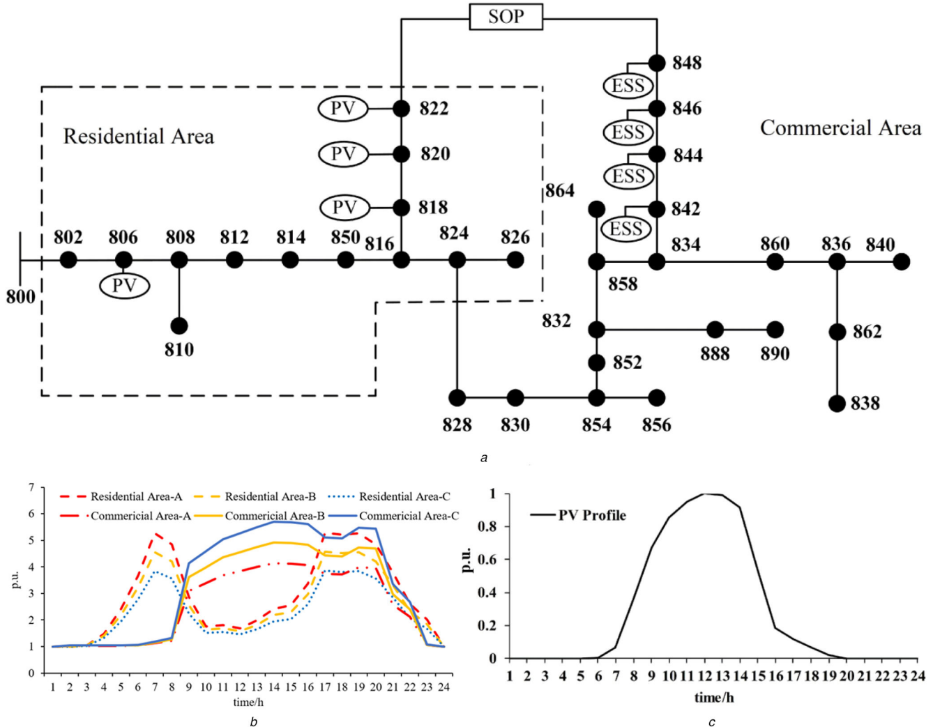
Fig. 3 Modified IEEE 34-node test feeder
